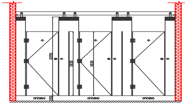
Front View (EU)
