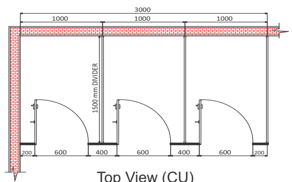
Top View (CU)
