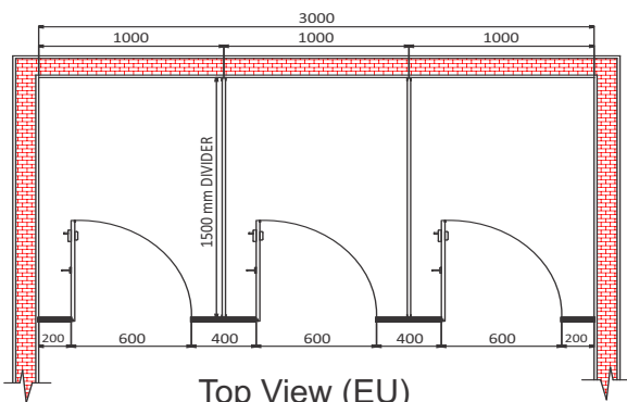
Top View (EU)
